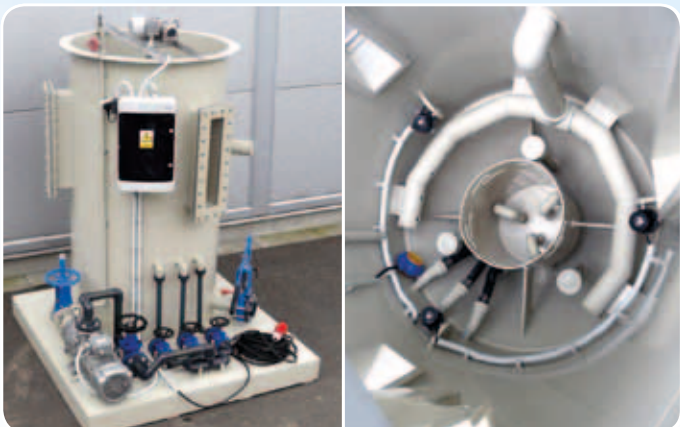
AS-FLOT Flotation Unit
